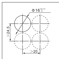
安装防护罩F-I头部的开孔 Drilling plan for operators with cap F-I
