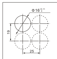
矩形头部开孔 Drilling plan for rectangular operators
