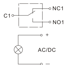
一常开一常闭 One normally open and one normally close, wiring diagram
