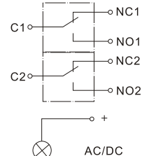
二常开二常闭 Two normally open and two normally close, wiring diagram
