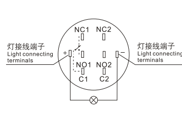
二常开二常闭 Two normally open and two normally close, wiring diagram
