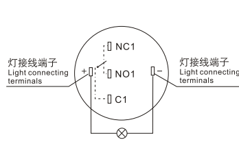
接线示意图 Light connecting terminals
