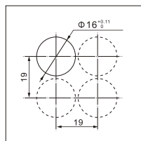
圆形/方形头部开孔 Drilling plan for round and square operators
