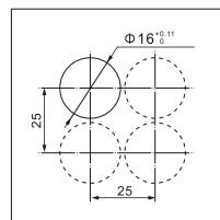
蘑菇头开孔 Drilling plan for mushroom button operators
