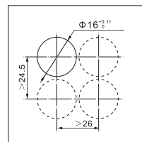
安装防护罩F-II头部的开孔 Drilling plan for operators with cap F-II
